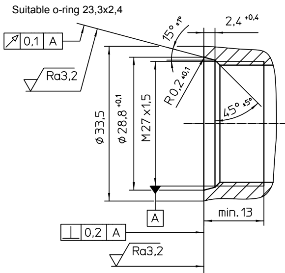
Fig. 11: Connection geometry to Type G RC Y 063 N54 A01
