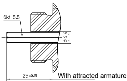
Fig. 10: Dimensional drawing to Type G RC Y 063 N54 A01
